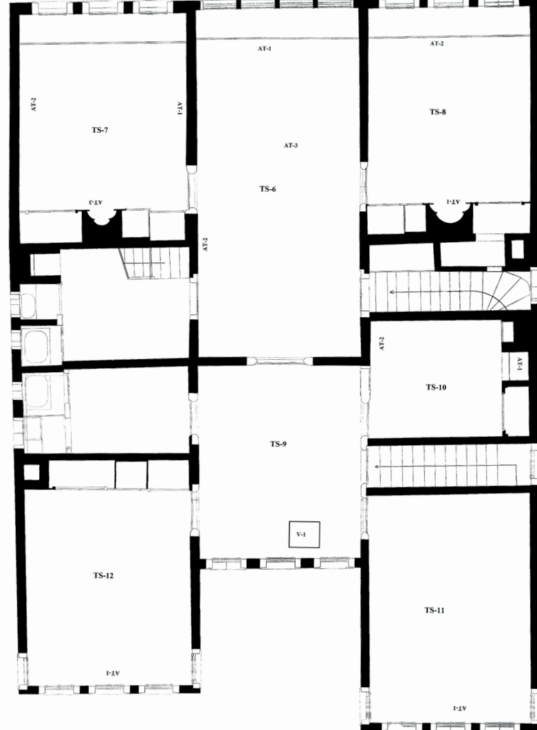
Tokat Atatürk House and Ethnography Museum First Floor Plan
