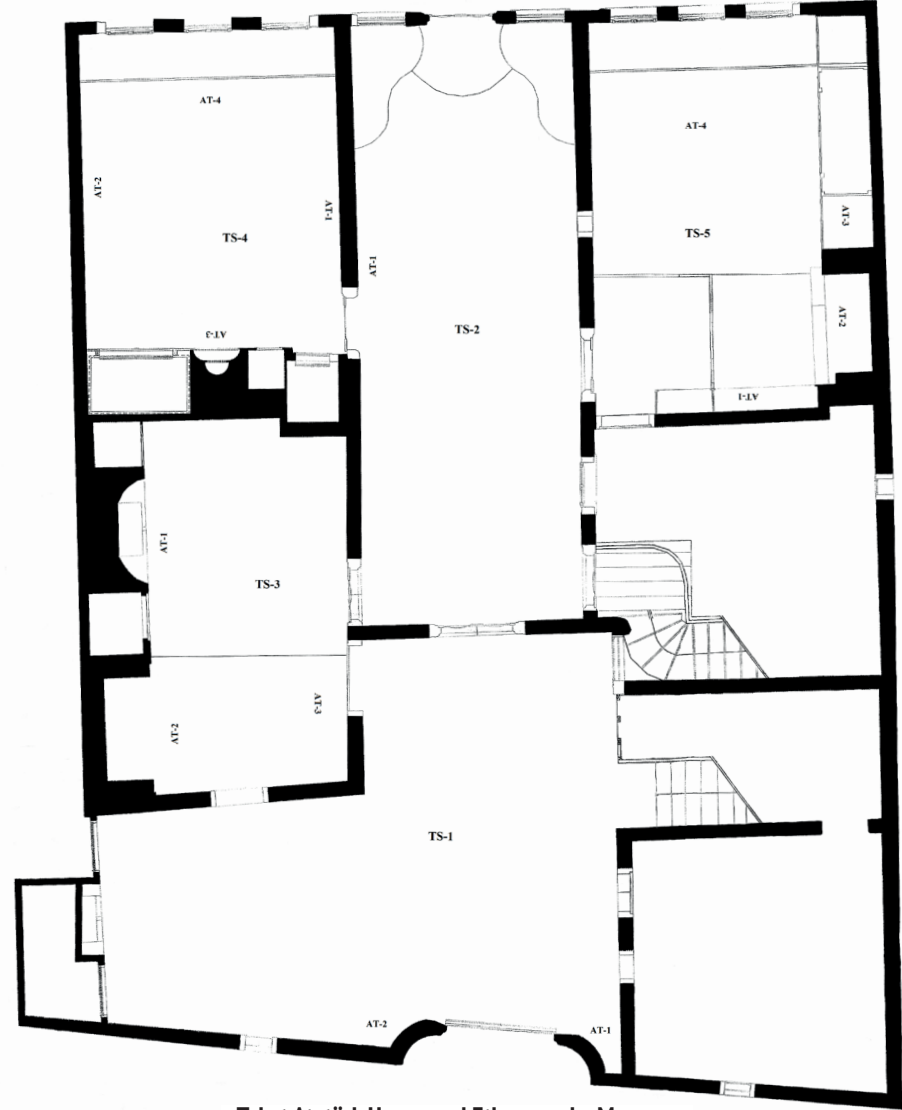
Tokat Atatürk House and Ethnography Museum Ground Floor Plan
